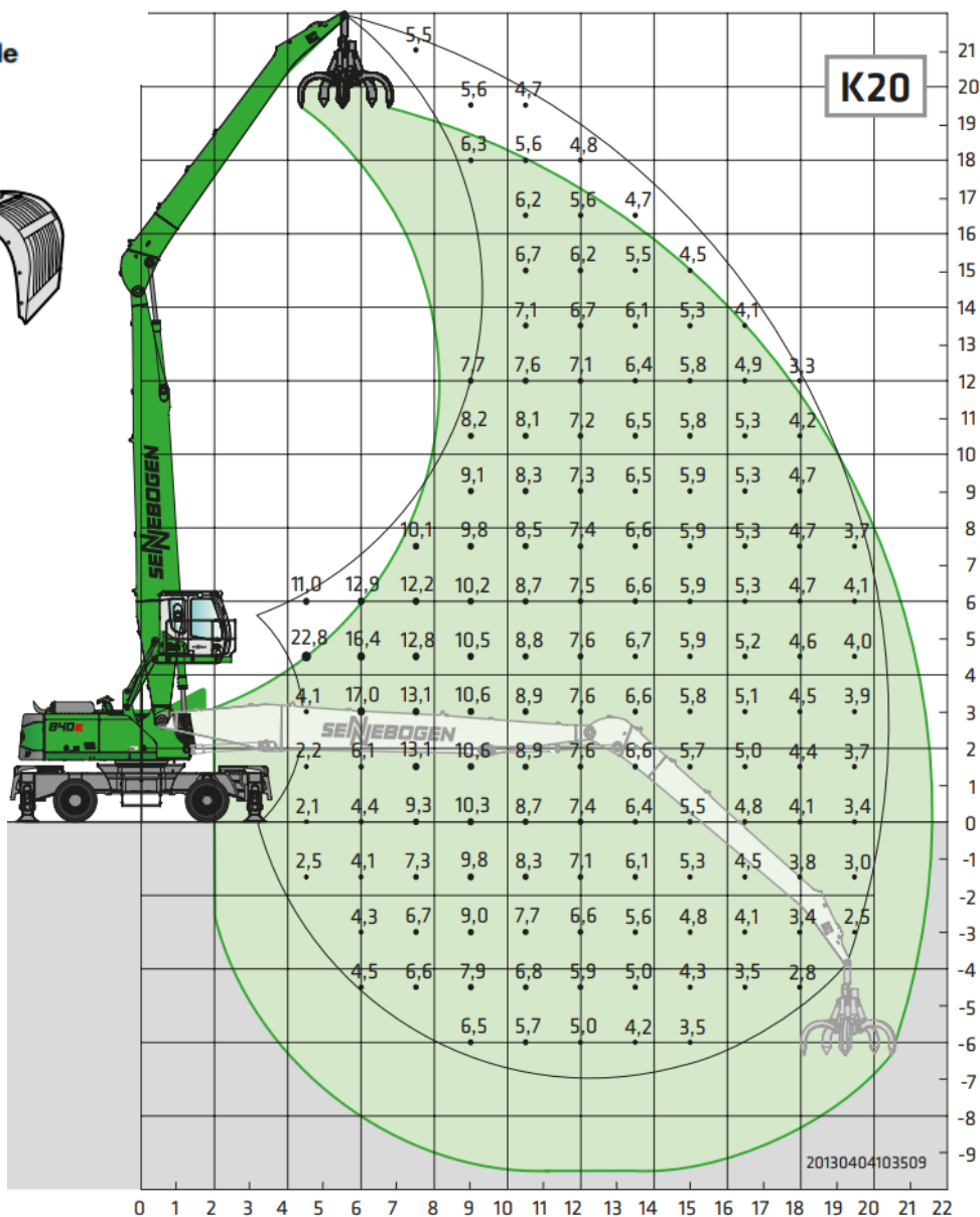
Recycling and Demolition Grab
