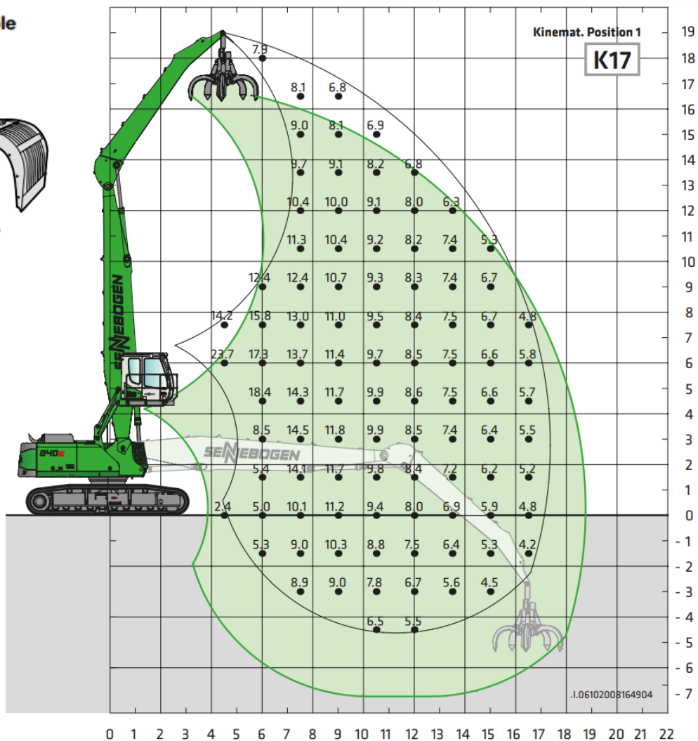
Recycling and Demolition Grab
